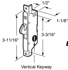
Vertical Keyway
