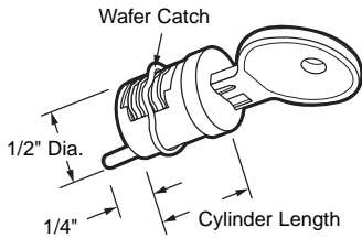
E-2005 (cylinder length - 13/16") E-2087 (cylinder length - 7/8") E-2088 (cylinder length - 1-1/4")
