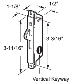
Vertical Keyway
